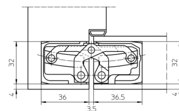
Blockzarge
