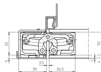
Stahlzarge
