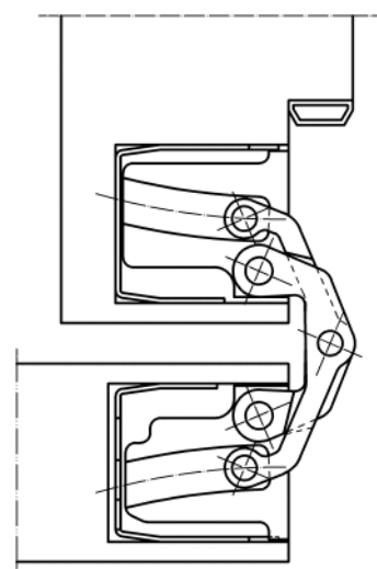
Blockzarge 180°
